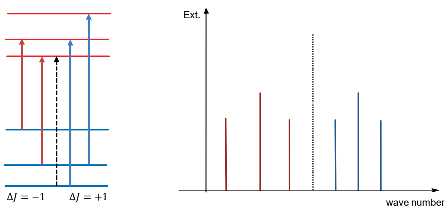
Figure 2.12.: Energy transitions (left) and corresponding rotational-vibrational spectrum of HCl (right), asymmetry caused by rotation-vibrational-coupling. Dotted line corresponds to the hypothetical transition \Delta J = 0 not found in the HCl-spectrum.
